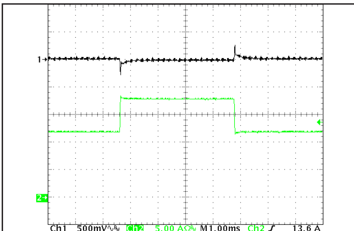
Figure 5: Output response to load current step for QTC version of product (50% - 75% - 50% of I out (max); dI/dt = 0.1 A/μs). Load cap: 15 μF tantalum cap and 1 μF ceramic cap. Ch 1: V out , Ch 2: I out .
